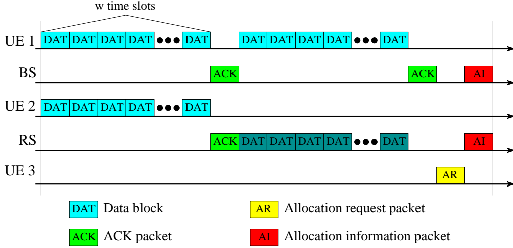
Figure 3.2: Time slot scheduling for the protocol with allocation based on local parameters, with k_r = 2 . UE 1 is allocated directly to the BS, UE 2 is helped by the relay RS, whereas UE 3 still has to determine its own allocation.
