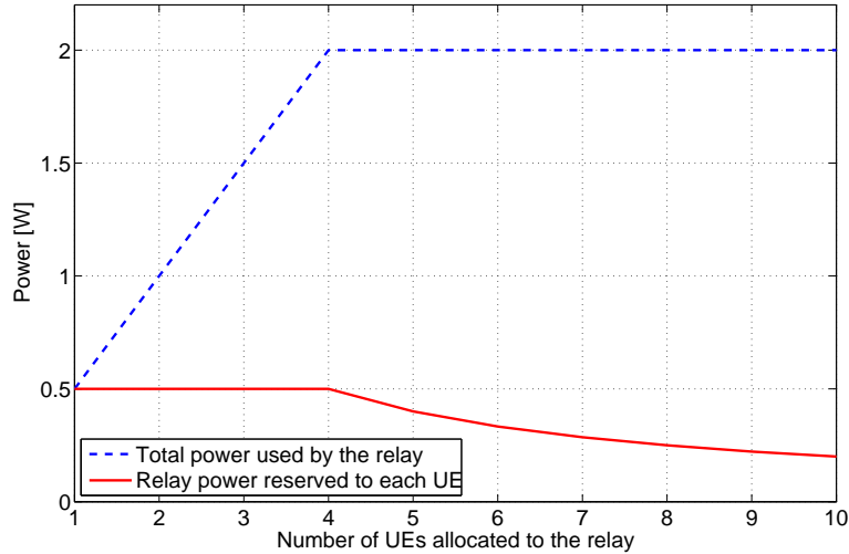
Figure 2.1: Power allocation at the relay, when P_t = 0.25 W, P_R = 2 W. We assume \eta = 2 , meaning that an amount of power equal to 2P_t is reserved to each relayed UEs, when their number is up to 4. Beyond that value, the relay uses its maximum power transmission, which is equally shared among all the UEs.
