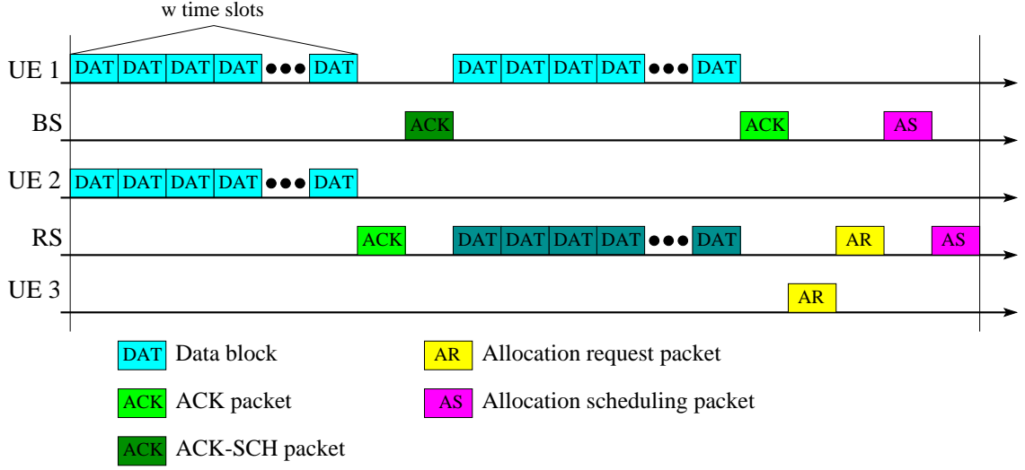
Figure 3.5: Time slot scheduling for the OAB protocol. UE1 is allocated to the BS, whereas UE2 is allocated to a relay. After the relays send the ACK packets, the BS transmits the ACK-SCH packet, in order to allow opportunistic forwardings and avoid collisions. UE3 has just joined the network, and uses the AR packets to retrieve its default allocation.
