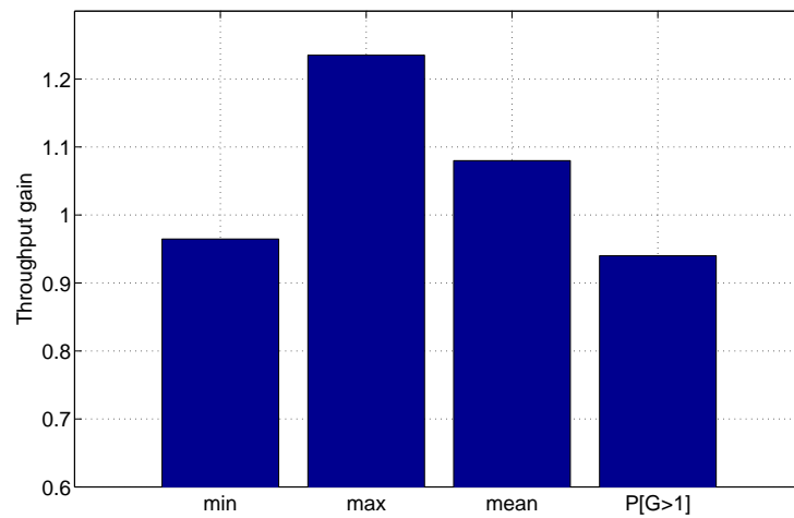
Figure 3.12: Throughput gain in a CDMA scenario, with SIC and OR. Allocation is done via the OAB protocol, implementing the GEO allocation algorithm.
